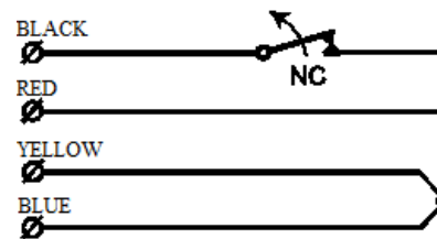
Circuit diagram – colour cables
