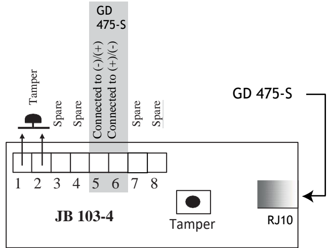
JB 103-4 Junction box with RJ10 connector for GD 475-S, opening protection switch
