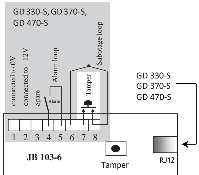
JB 103-6 Junction box with RJ12 connector for GD 330-S, GD 370-S and GD 470-S, opening protection switch
